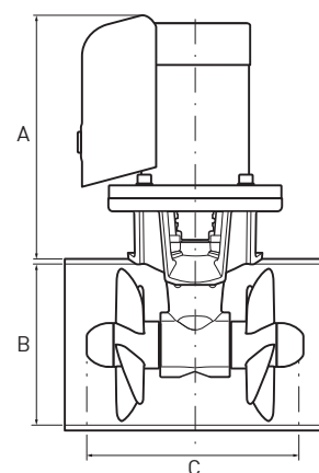
Double Propeller
