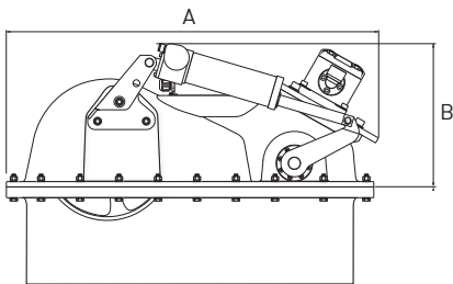
DC Retractable Thrusters Diam. 185 mm
