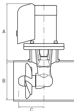
Single Propeller
