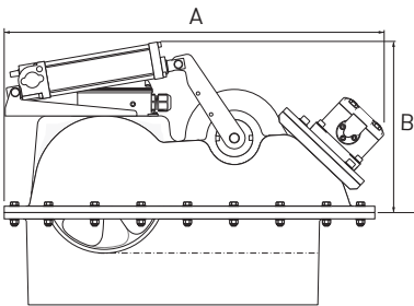
Hydraulic Retractable Thrusters Diam. 185 mm
