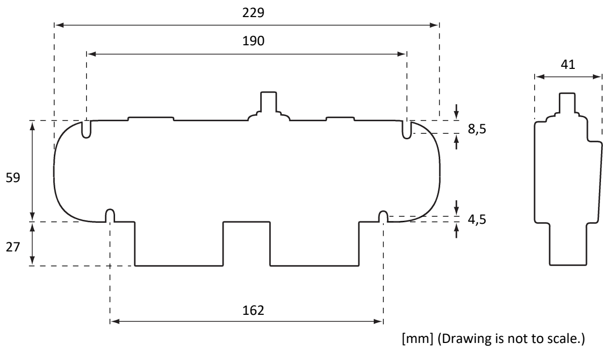
Figure 5.1: Dimensions
