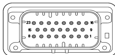
View looking at back of the display Mating connector P/N: AMP 770680-1
