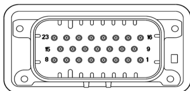
View looking at back of the display Mating connector P/N: AMP 770680-4
