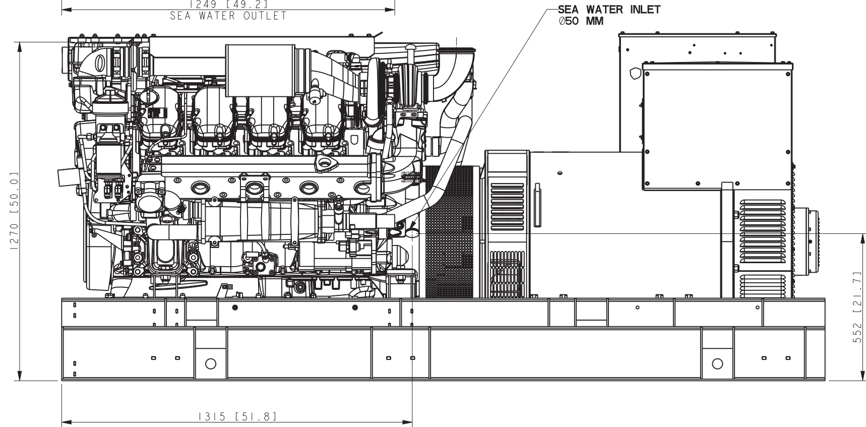
ENGINE WITH HEAT EXCHANGER AND SINGLE FUEL/ OIL FILTER
