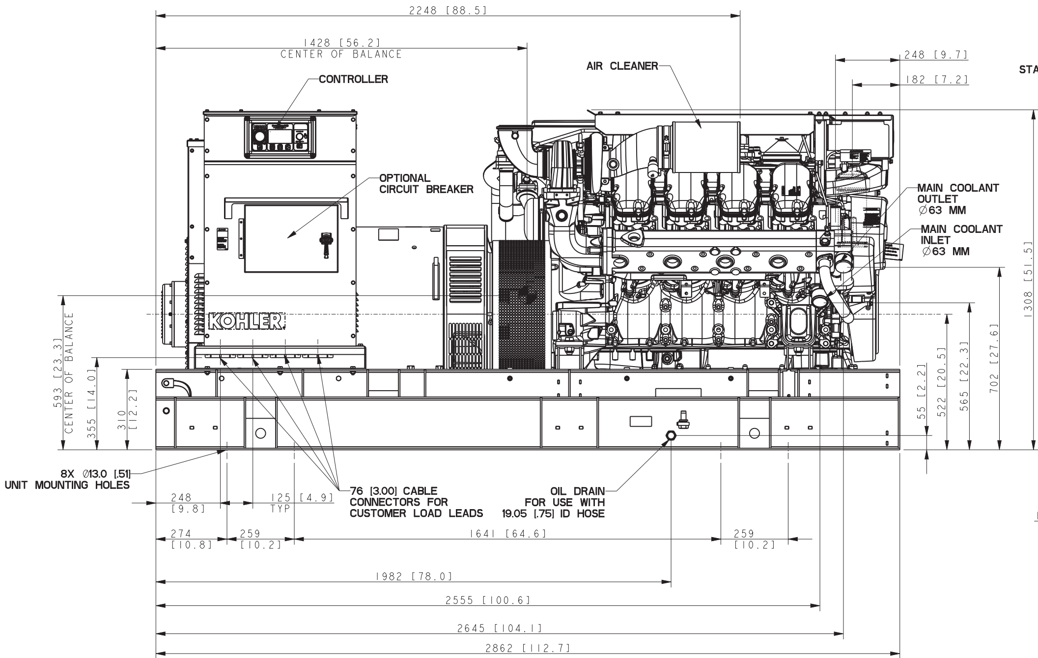
ENGINE WITH KEEL COOLING AND SINGLE FUEL/ OIL FILTER
